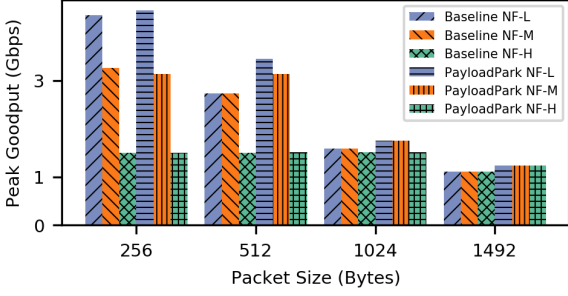
Figure 15: (Higher is better) Goodput with different NFs: NF-Light, NF-Medium and NF-Heavy.
