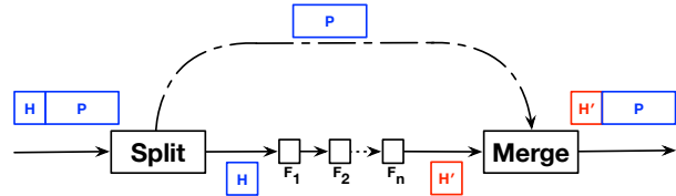
Figure 1: Abstract PayloadPark deployment. Split decouples the packet into header H and payload P . The header H is then processed by a shallow NF chain F_1, F_2 \dots F_n . Merge reassembles the resulting header H' with payload P .
