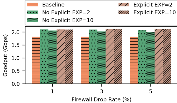
Figure 12: (Higher is better) Goodput using Explicit and No Explicit Drop packets for Firewall \rightarrow NAT . EXP=2 and EXP=10 labels denote Expiry threshold of 2 and 10 respectively. Standard error in goodput measurements is less than 0.26Mbps. The graph shows that PayloadPark has better goodput than baseline.
