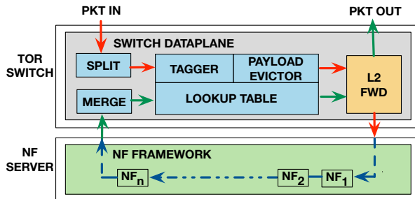
Figure 3: Packet flow in PayloadPark. Split decouples the packet header and payload and stores the payload in the payload table. The Merge operation merges the headers from the NF server with the payloads stored in the lookup table. L2 FWD forwards packet using L2 forwarding.
