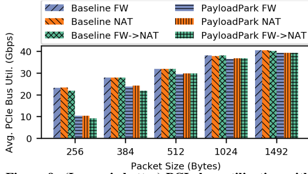
Figure 9: (Lower is better) PCIe bus utilization with different packet sizes.
