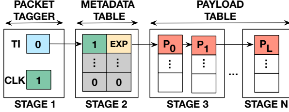
Figure 4: PayloadPark dataplane implementation. Packet processing proceeds from stage 1 to stage N. Packets are first tagged, then looked up in the metadata table, and finally stored in the payload table. The tagger has registers for the table index (TI), which is an index into the metadata and payload tables, and a clock (CLK). The metadata table contains two values at each index, the value of the clock when the index was occupied and an expiry threshold (EXP). If the index is available for storing payload, its EXP value is 0. Payload blocks ( P_0, P_1 \dots P_L ) are striped across MATs.
