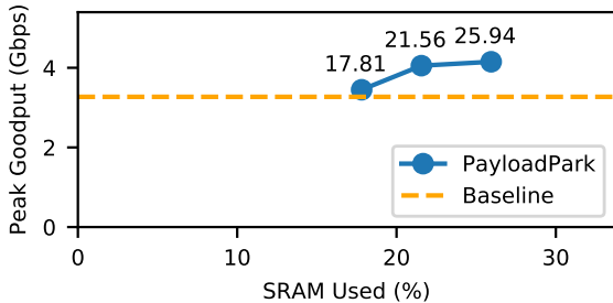
Figure 14: (Higher is better) Goodput compared to percentage of reserved memory on the Tofino chip. Labels on points show specific memory usage.
