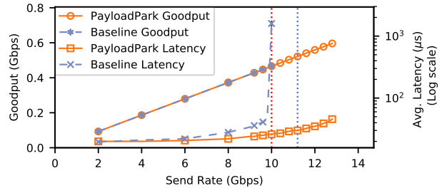
Figure 13: Goodput and latency improvements of PayloadPark with FW \rightarrow NAT \rightarrow LB chain on NetBricks. This is the recirculation-enabled version of the experiment described in Fig. 7.
