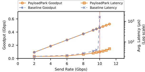
Figure 7: Results for FW \rightarrow NAT \rightarrow LB . The vertical red line at X=10 Gbps highlights baseline link capacity. For X < 10 Gbps, the maximum difference between peak and average latency is 0.66 \mu s for baseline and PayloadPark. At X=10 Gbps, this difference is 21 \mu s and 0.66 \mu s for baseline and PayloadPark, respectively.
