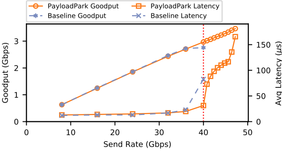
Figure 16: Goodput and latency of PayloadPark and Baseline with 512 byte packets and Firewall → NAT chain. The vertical red line at X=40 Gbps highlights baseline link capacity.
