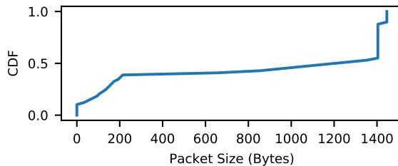
Figure 6: Packet size distribution for simulating enterprise datacenter traffic pattern.
